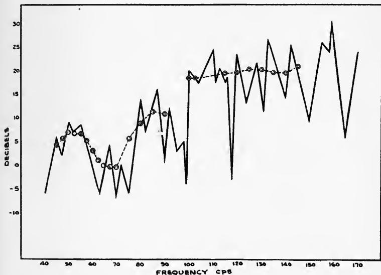
FIG. 5. Calculated response using complex signal. Solid lines join points measured using sinusoidal signal; circle points: "mean" calculated for bands 10 cps wide below 100 cps and 25 cps wide above 100 cps.
